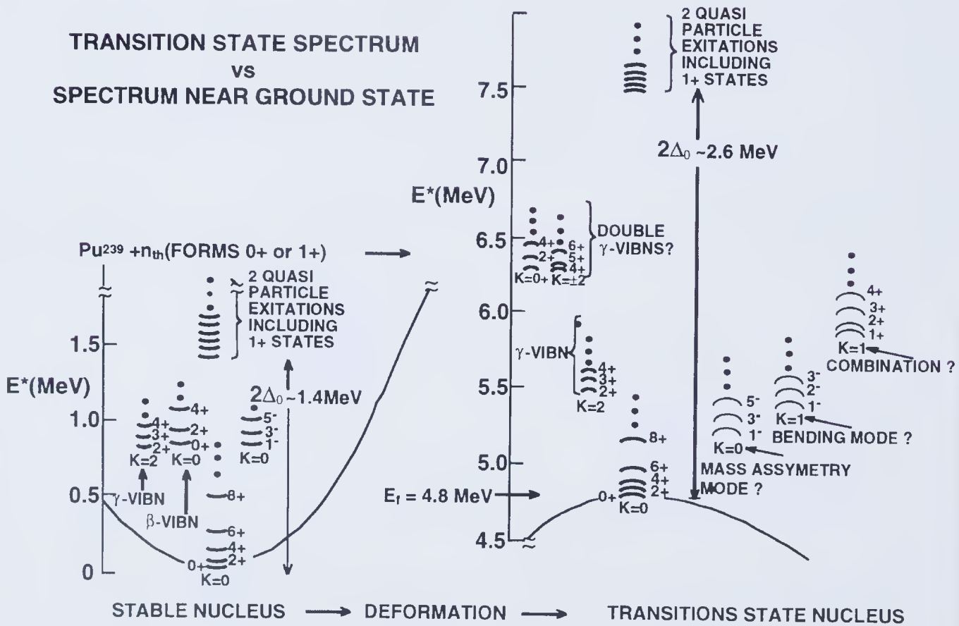
Figure 2. Comparison of transition states at the fission barrier with the spectrum of low lying states for deformed nuclei (modified from Griffin 1965).
